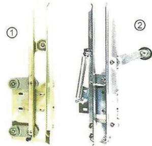
Car Door Clutch
