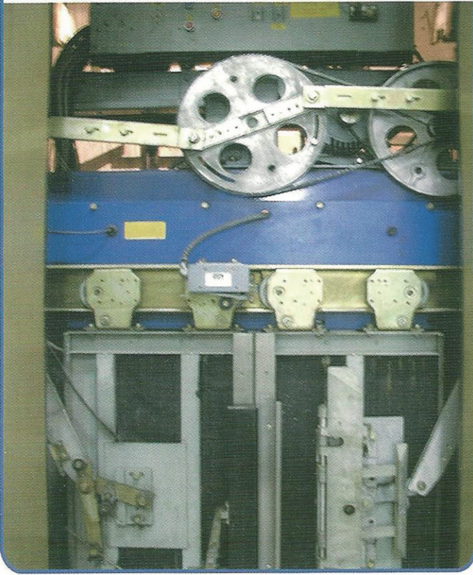
Car Door
