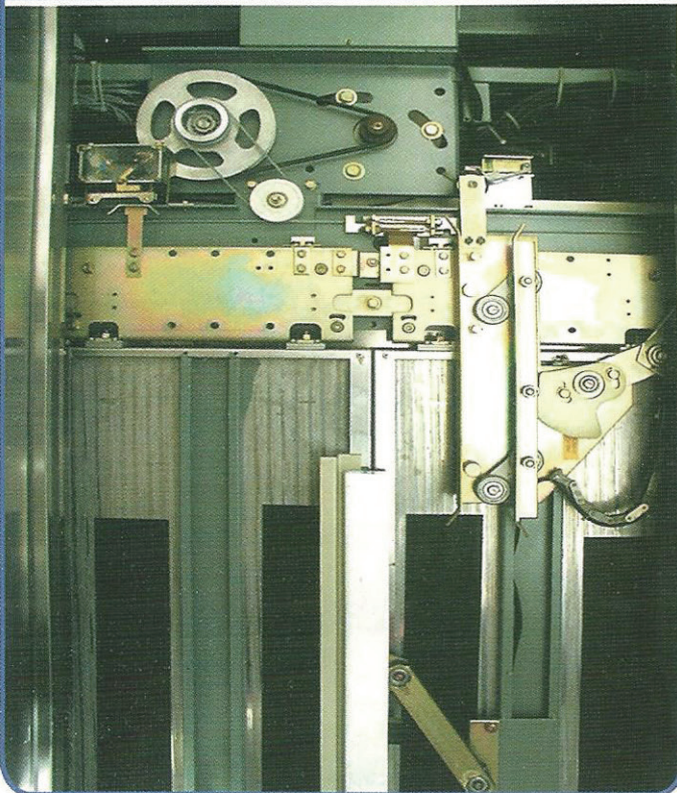
Car Door
